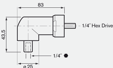
0 607 453 630 Dimensions in mm
