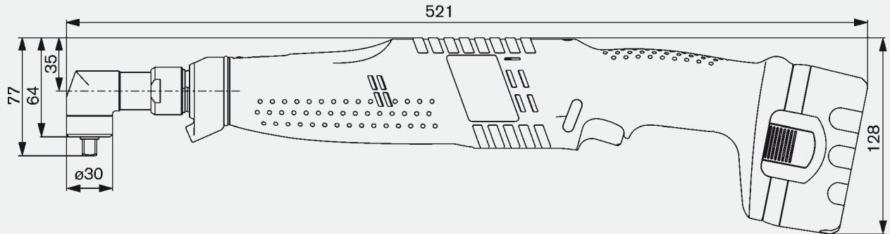
ANGLE EXACT models: 17, 23, 30, 22 CF, 29 CF all 14.4 volt models Dimensions in mm
