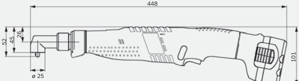
ANGLE EXACT models: 2, 3, 6, 7, 8, 15, 14 CF; all 9.6 volt models Dimensions in mm
